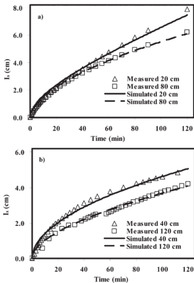
Fig. 4. The cumulative infiltration ( I_s ) curves of (a) measured and simulated infiltration at Site 4 under double-ring infiltrometers for inner-ring diameters ( d_i ) of 20 and 80 cm, and (b) measured and predicted infiltration at Site 4 under double-ring infiltrometers for d_i of 40 and 120 cm.
