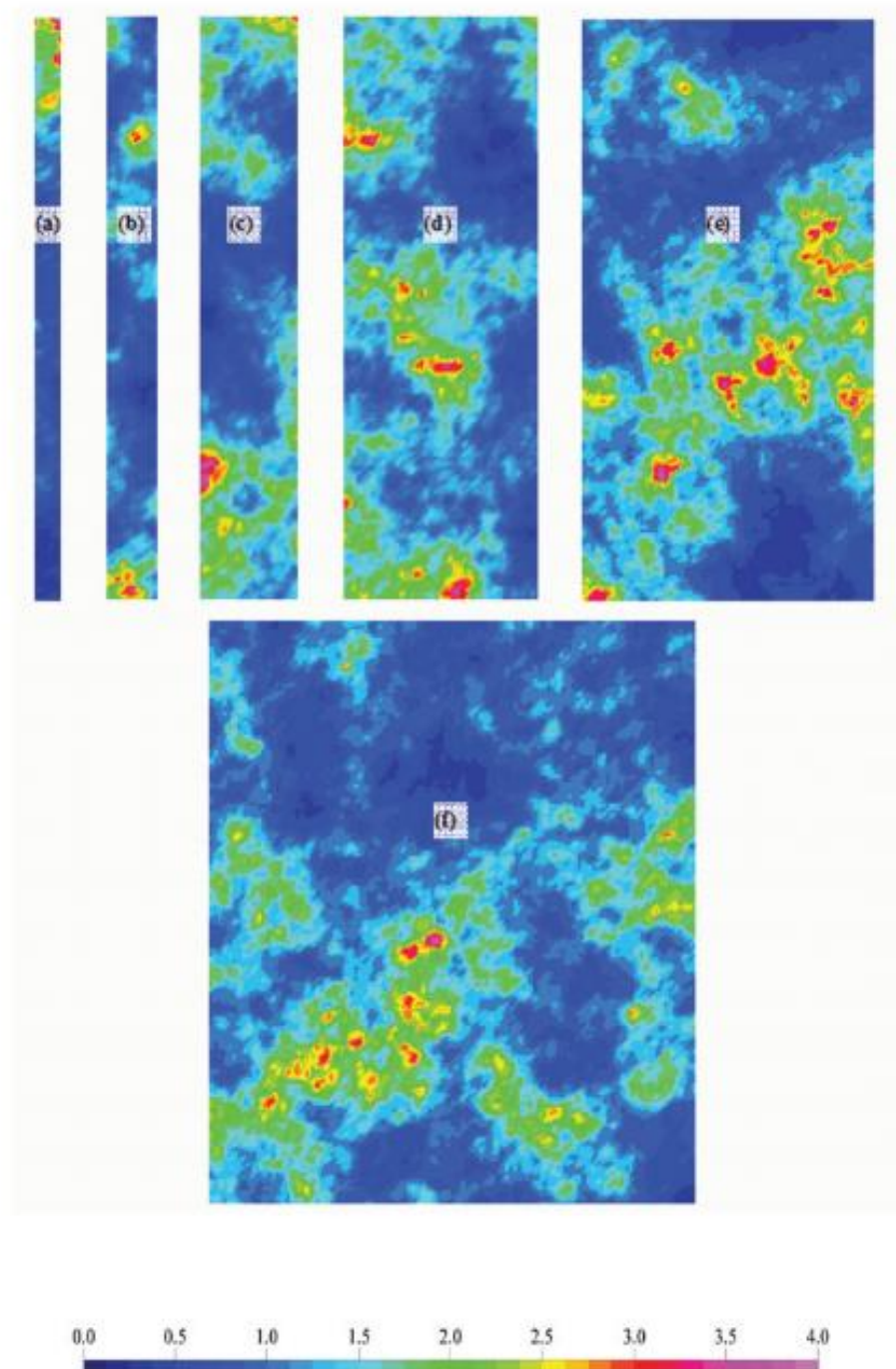
Fig. 8. Representative maps of scaling factor fields (correlation length L = 20 cm, SD = 0.25 ) for different diameters: (a) 10 cm, (b) 20 cm, (c) 40 cm, (d) 80 cm, (e) 120 cm, and (f) 200 cm.
